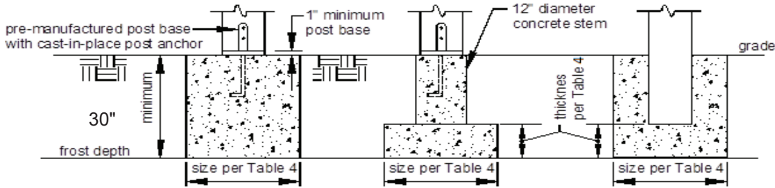
FIGURE 10: FOOTINGS
