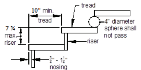
FIGURE 33: TREADS AND RISERS
