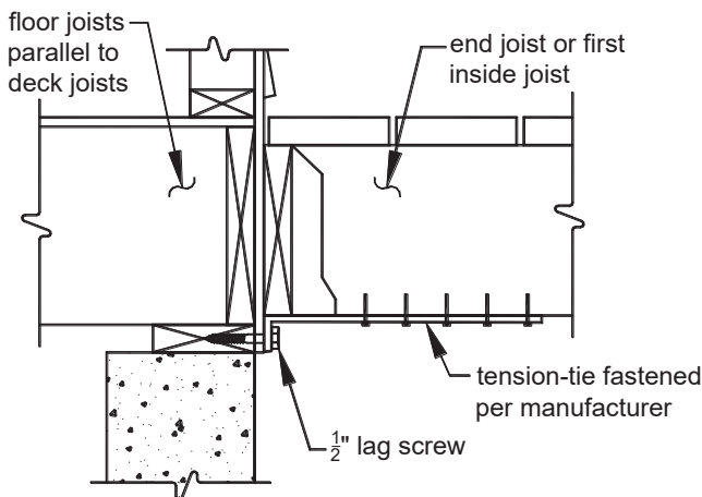
FIGURE 21: TENSION-TIE CONNECTION
