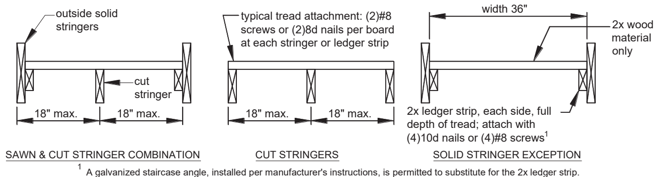
FIGURE 36: STRINGER TREADS
