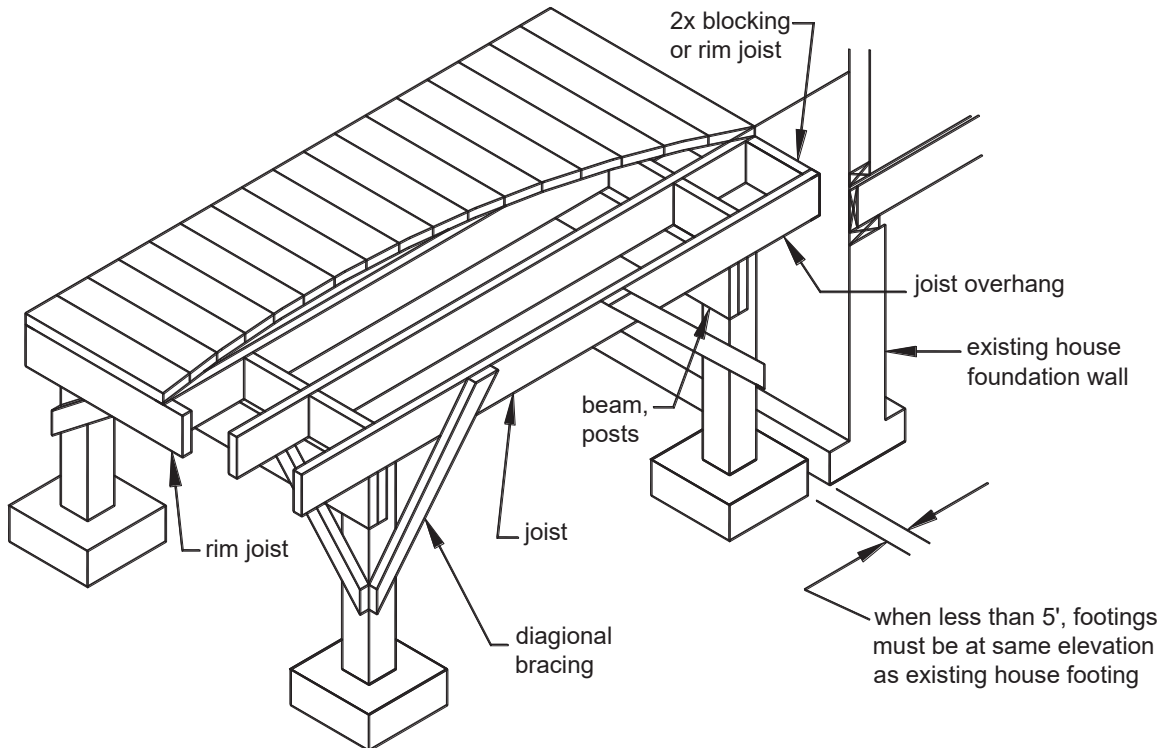
FIGURE 19: FREE-STANDING DECK
